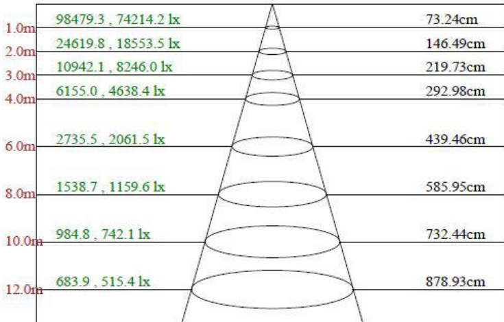
Max , Ave Beam angle of C337.5plane40.06
